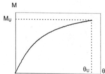
(b) Ultimate moment capacity ( M_U )
