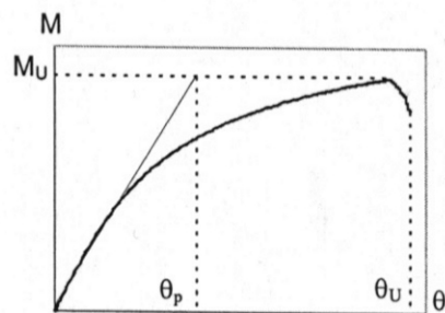
(b) Ultimate moment capacity ( M_U )
