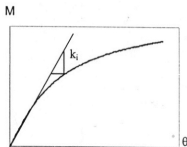
(a) Initial stiffness ( k_i )
